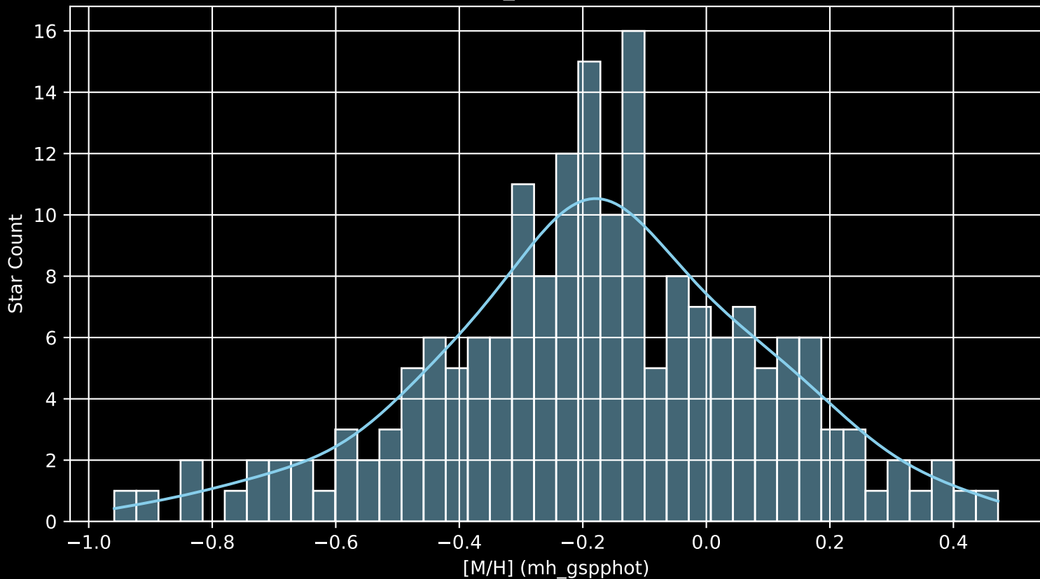
APOGEE DR17 Field: [INTCL_N6341_MGA [M/H] (mh_gspphot) (n= 184)
