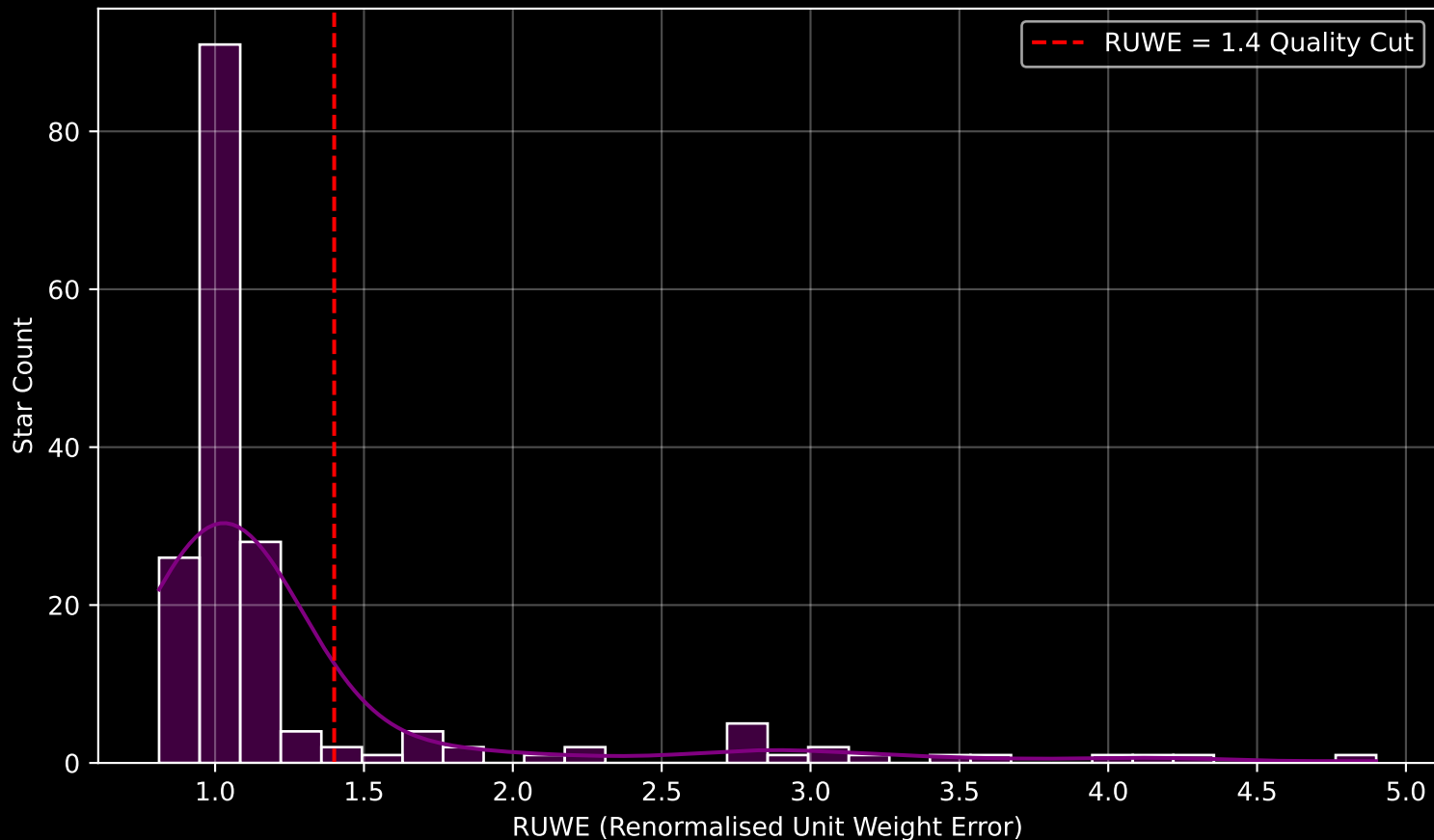
GAPOGEE DR17 Field [INTCL_N6341_MGA] RUWE Distribution (n= 176)
