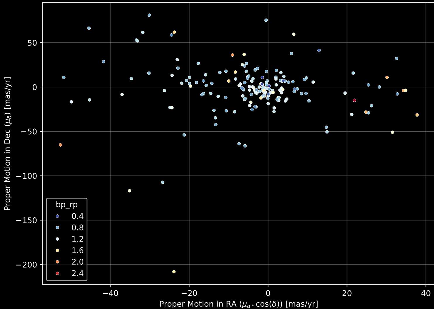
APOGEE DR17 Field: [INTCL_N6341_MGA] Proper Motion Diagram (n= 185)
