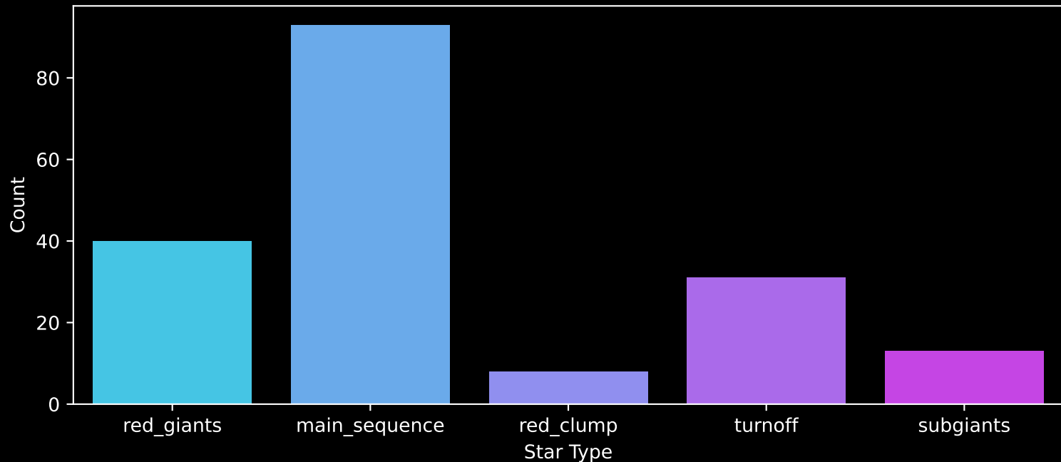
APOGEE DR17 Field: [INTCL_N6341_MGA] Count plot of Star Type
