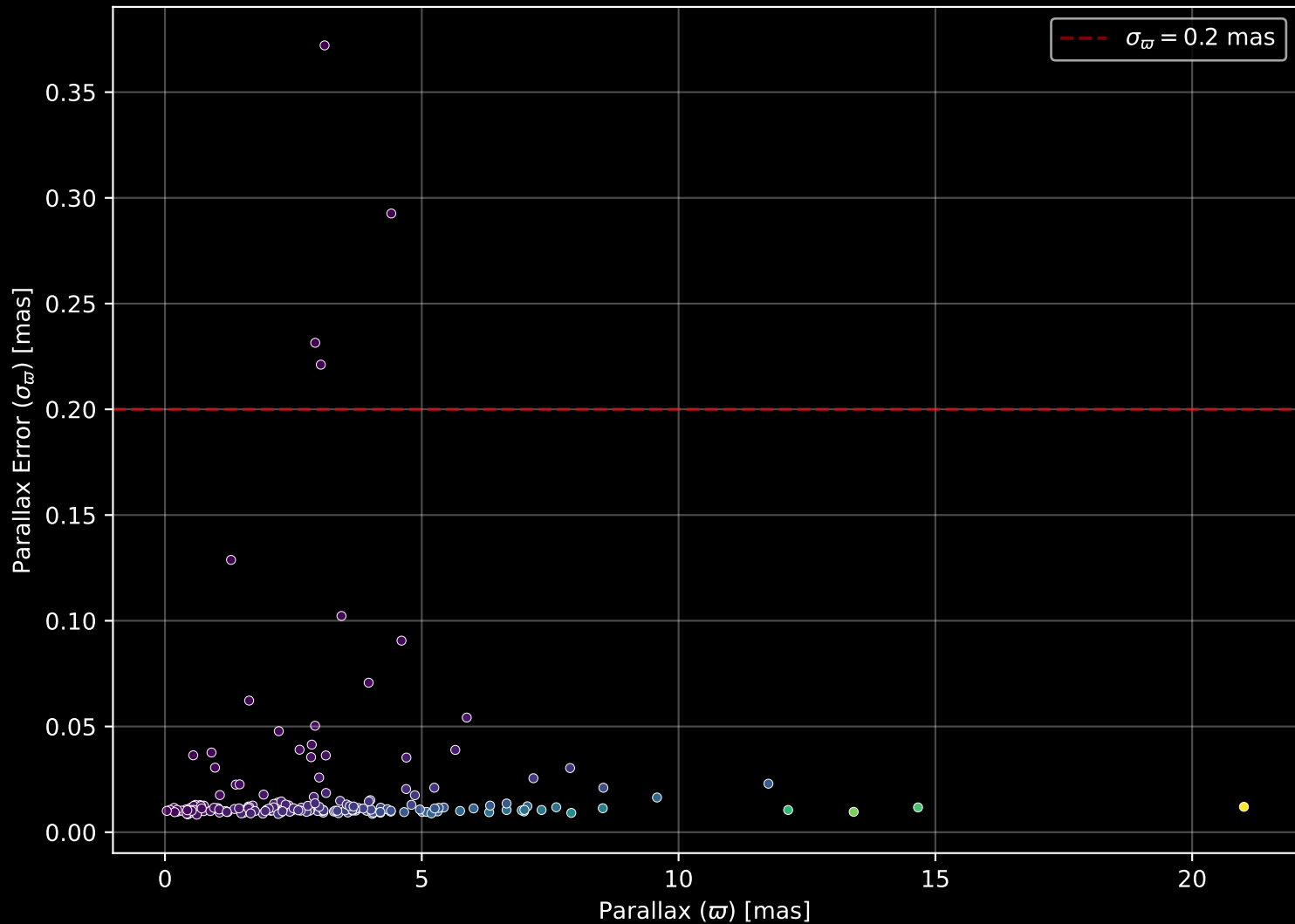
APOGEE DR17 Field: [INTCL_N6341_MGA] Parallax Quality (n= 185)
