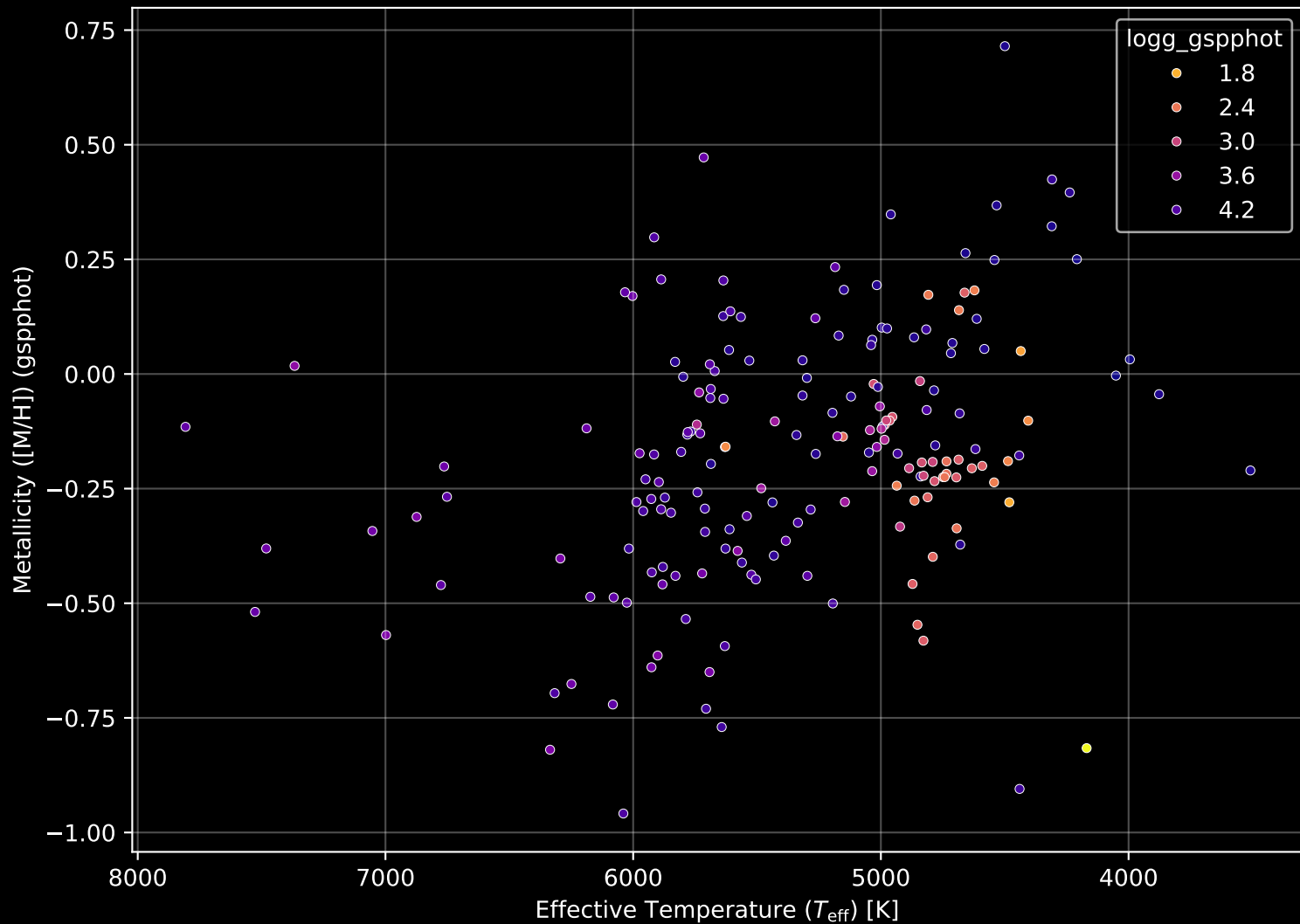
APOGEE DR17 Field: [INTCL_N6341_MGA] Stellar Population Parameters (n= 185)
